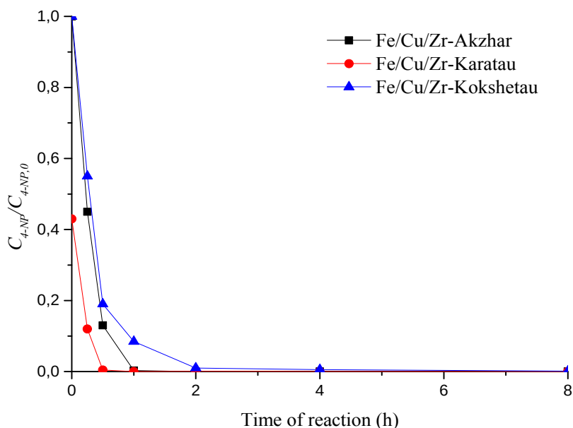
Figure 2 - Catalytic wet peroxide oxidation of 4-NP using the trimetallic PILCs. Operating conditions: C_{4-NP,0} = 5 g/L, CH_2O_{2,0} = 17.8 g/L, catalyst load = 2.5 g/L, initial pH 3.0 and T = 50 °C
